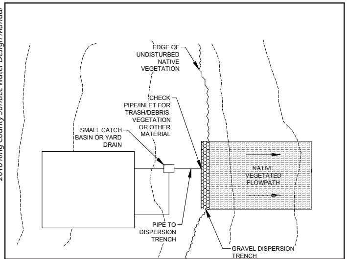
Roof application for gravel dispersion trench.
