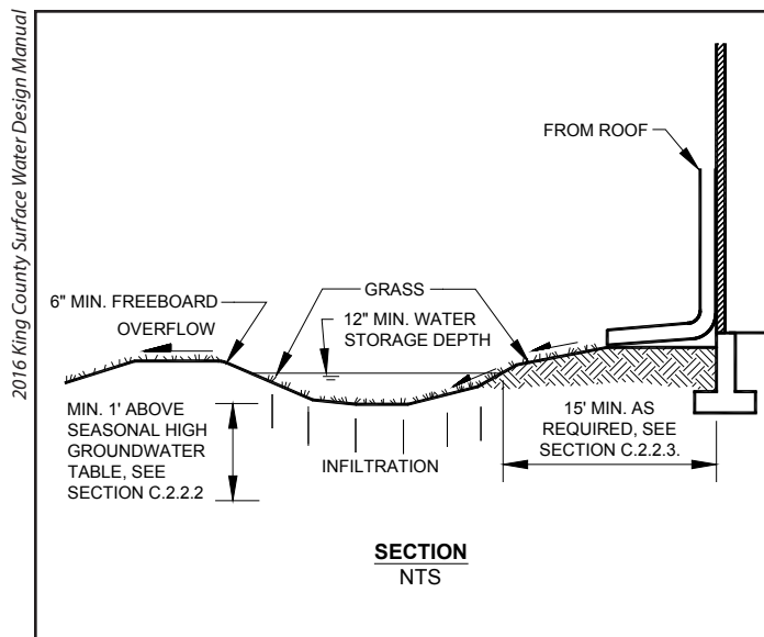
Typical ground surface depression infiltration system.
