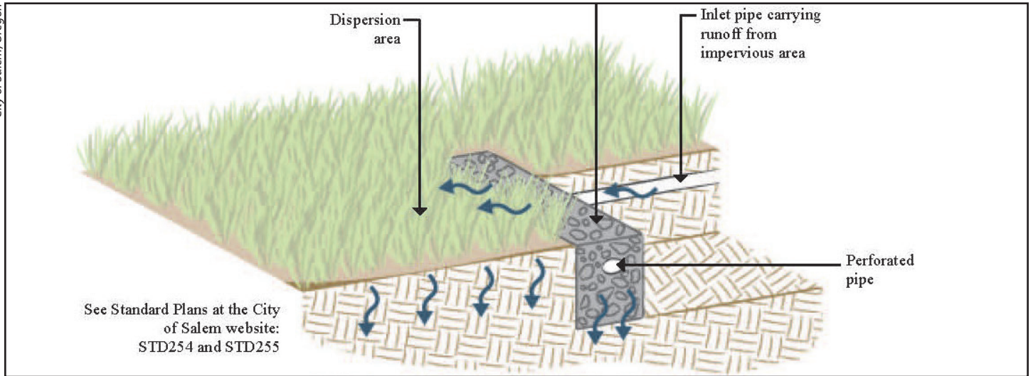
Graphic - example of a dispersion trench.
