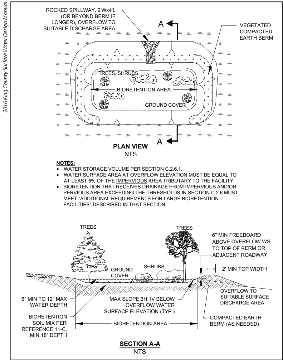
Plan and section view of a typical bioretention cell.
