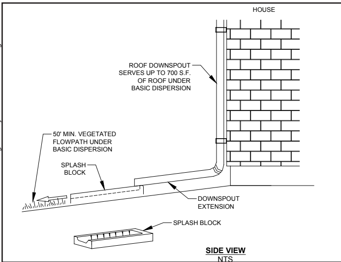
Typical Splashblock for Basic Dispersion
