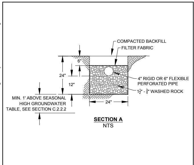
Typical trench infiltration system.
