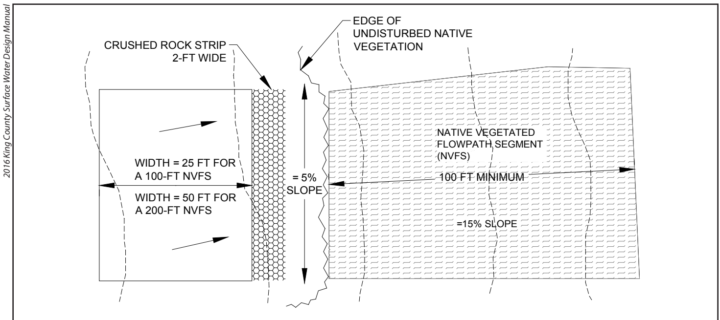
Application of sheet flow dispersion.
