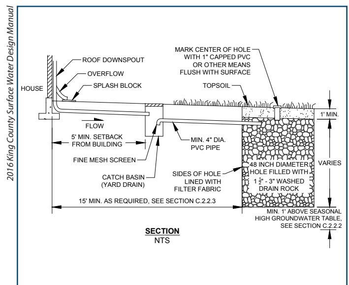
Typical drywell infiltration system.
